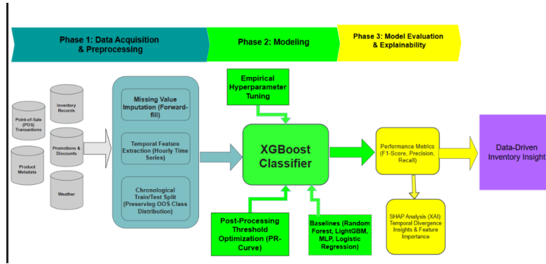
Fig. 1. The proposed algorithmic pipeline, illustrating the end-to-end transition from multi-source data preprocessing to machine learning classification and model evaluation.
